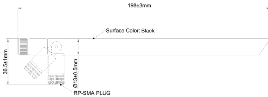
Figure 6: LoRa Antenna Dimension (mm)
