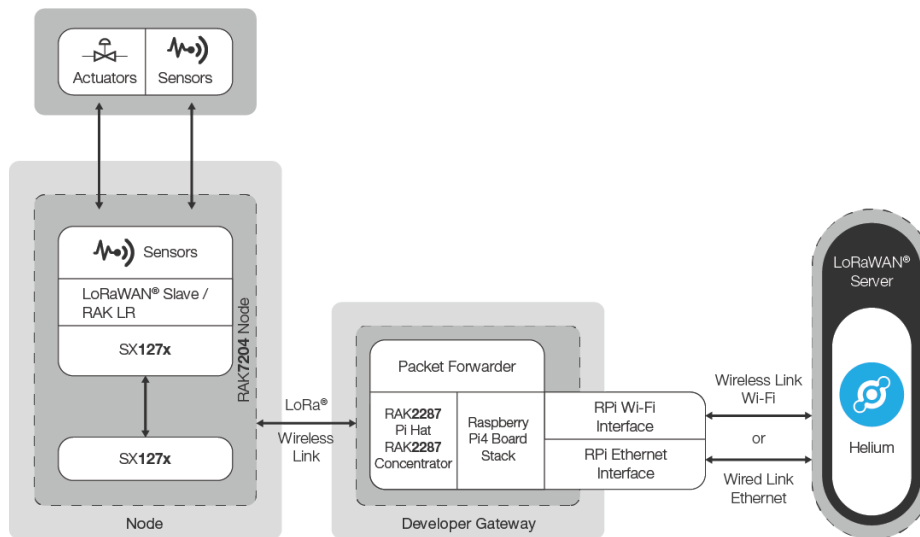
Figure 2: RAK Hotspot Miner System Structure
