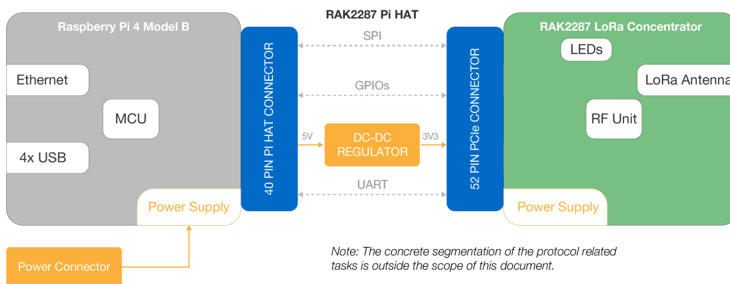
Figure 3: RAK Hotspot Miner Block Diagram
