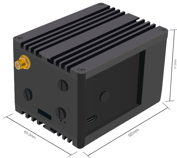
Figure 1: Device Dimensions
